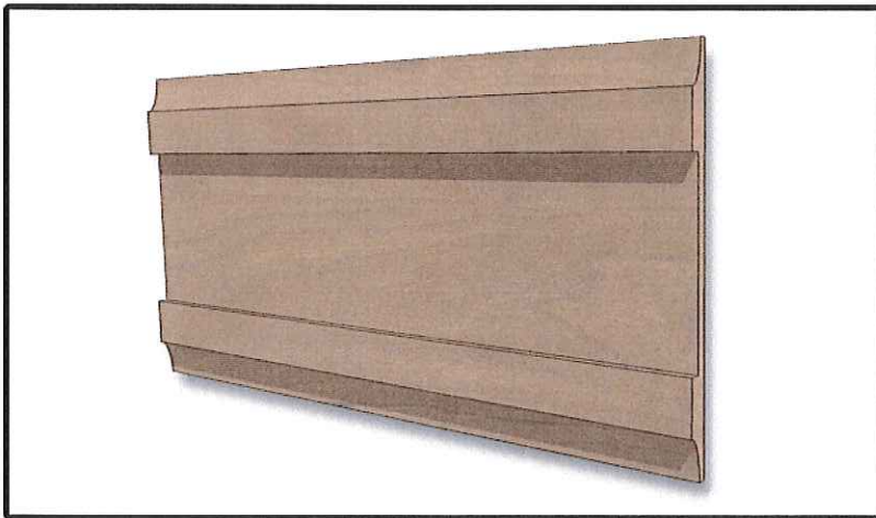
Tool Number: 4632 Description: Fascia Size: 7/8" X 7" Insert width: 3 1/2" Insert depth: 0.1875
