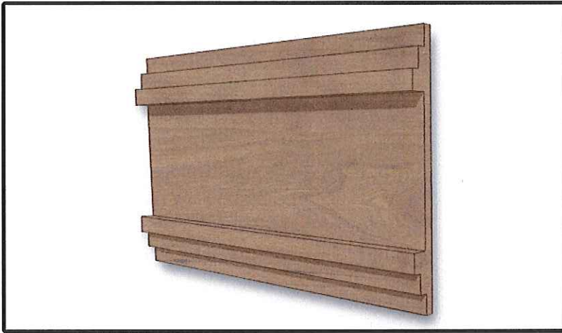
Tool Number: 4443 Description: Fascia Size: 1/2" X 5 1/2" Insert width: 3" Insert depth: 0.3125"
