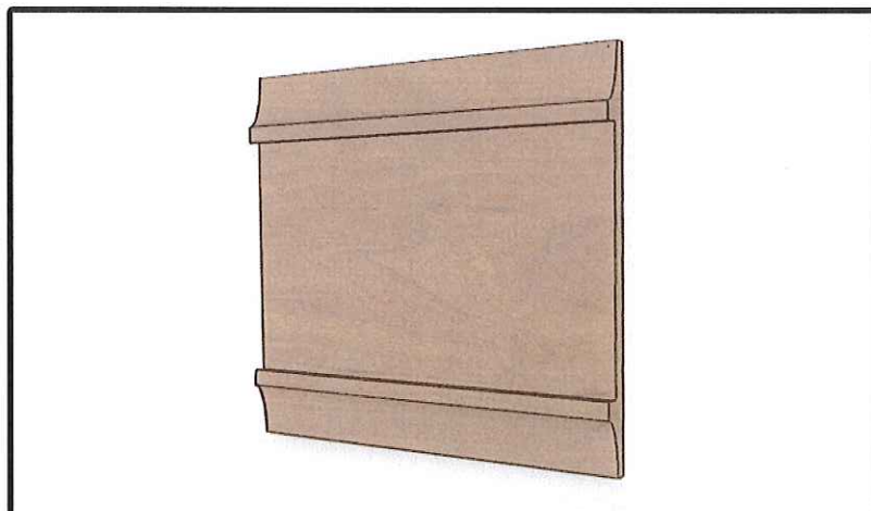
Tool Number: 4259 Description: Fascia Size: 3/8" X 5 1/2" Insert width: 3 1/2" Insert height: 3/16"
