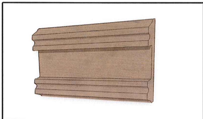
Tool Number: 4347 Description: Fascia Size: 1/2" X 4 1/4" Insert Width: 1.717"
